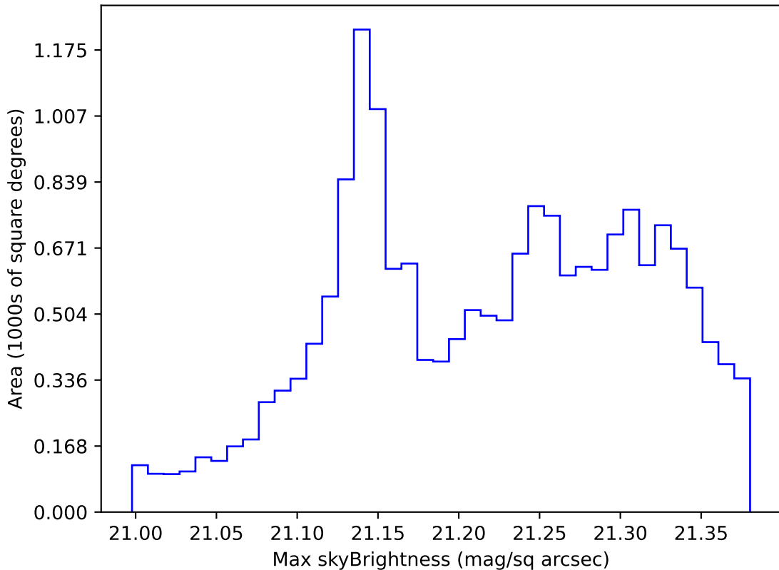
baseline_v3.5_10yrs WFD r band: Max skyBrightness
