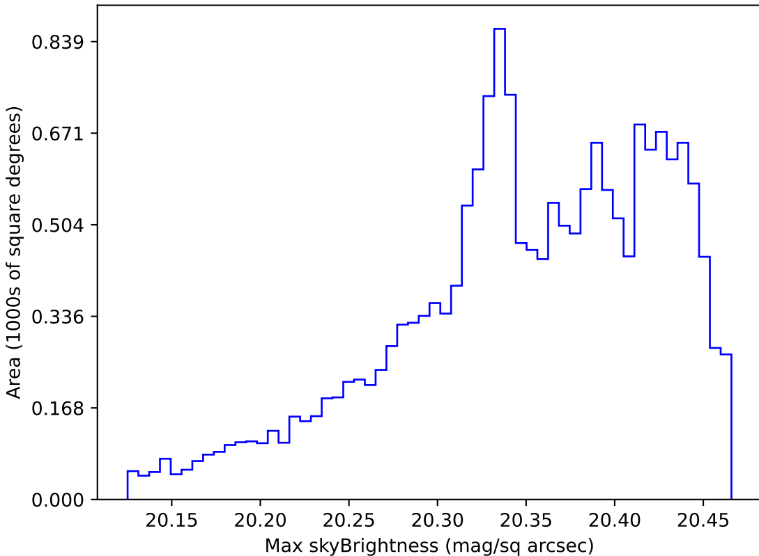
baseline_v3.5_10yrs WFD i band: Max skyBrightness
