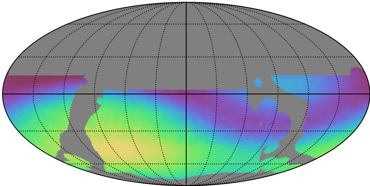
baseline_v3.5_10yrs WFD g band: Max skyBrightness
