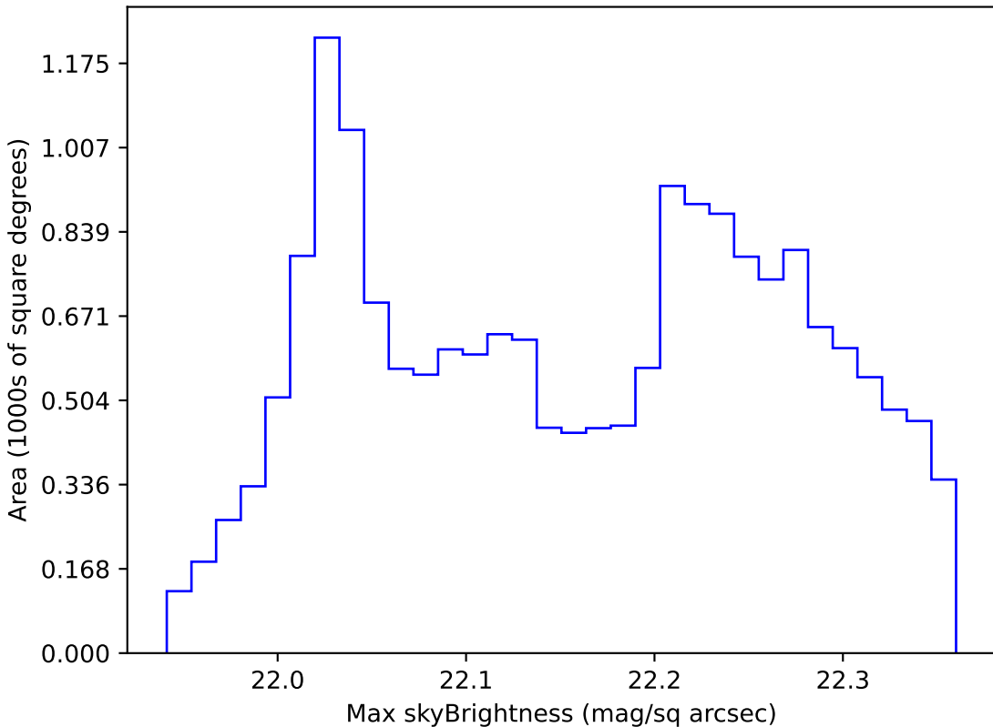
baseline_v3.5_10yrs WFD g band: Max skyBrightness
