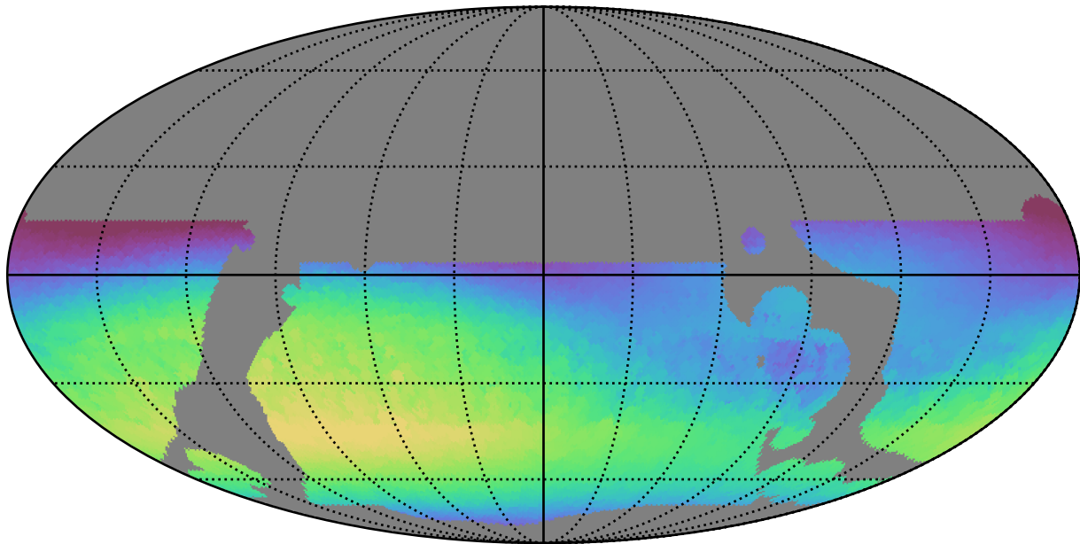
baseline_v3.5_10yrs WFD all bands: Max skyBrightness
