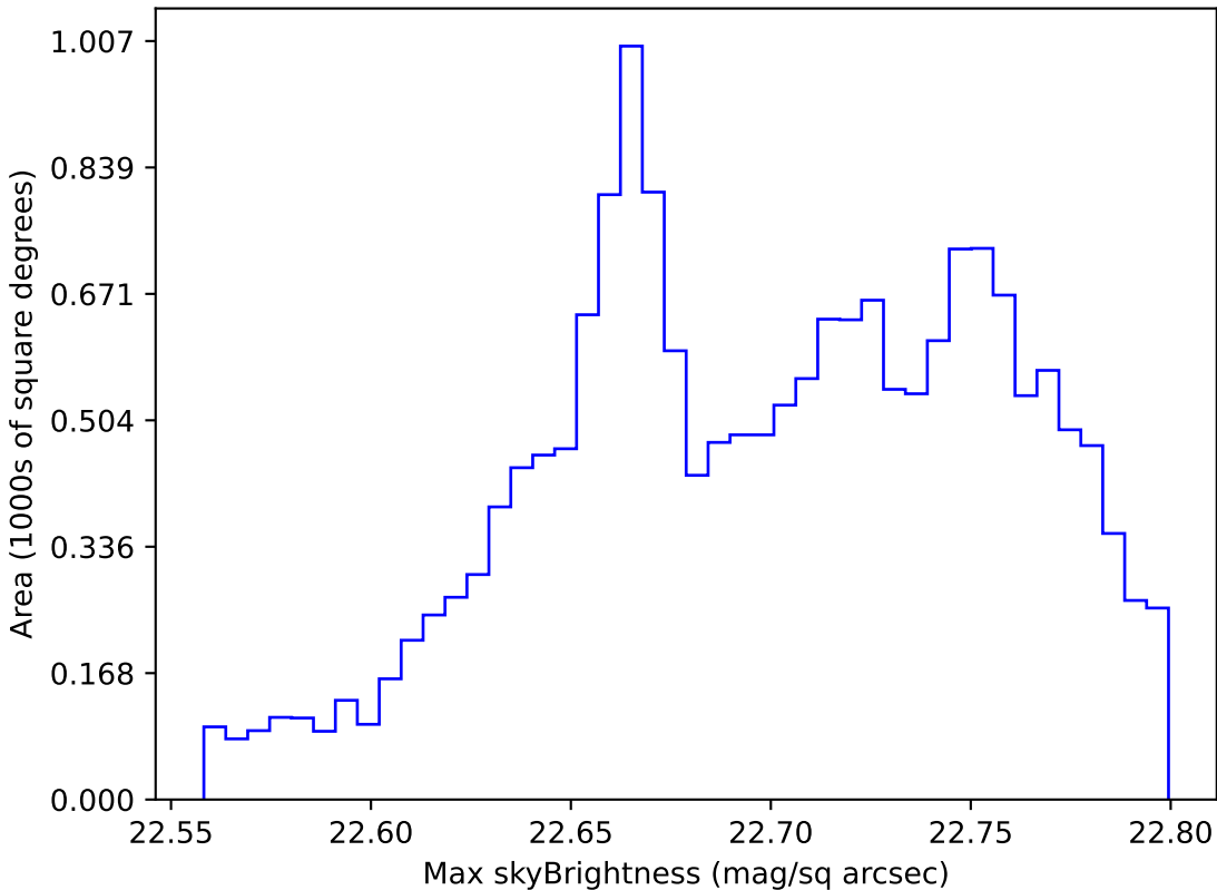
baseline_v3.5_10yrs WFD all bands: Max skyBrightness
