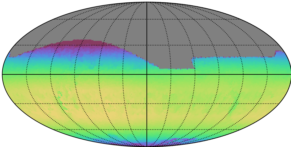
baseline_v3.5_10yrs All sky z band: Max skyBrightness
