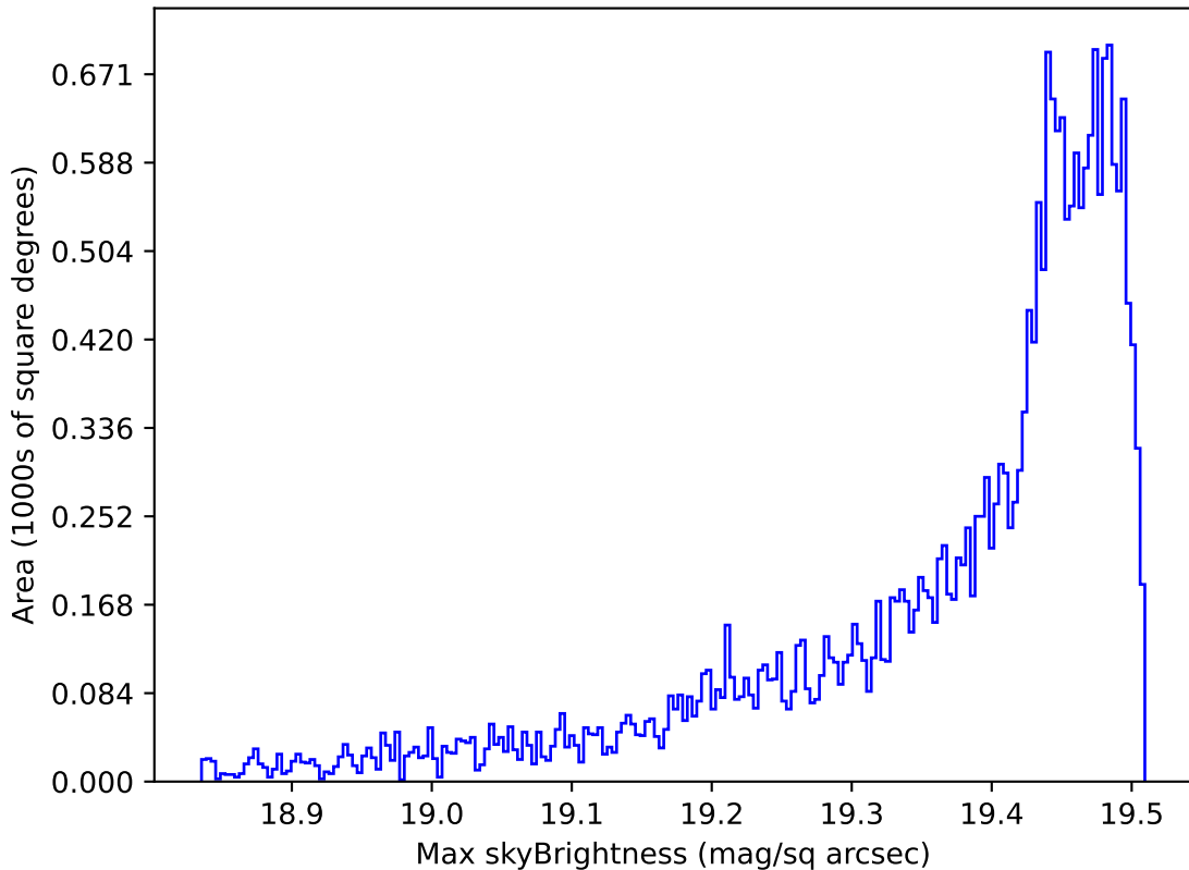
baseline_v3.5_10yrs All sky z band: Max skyBrightness
