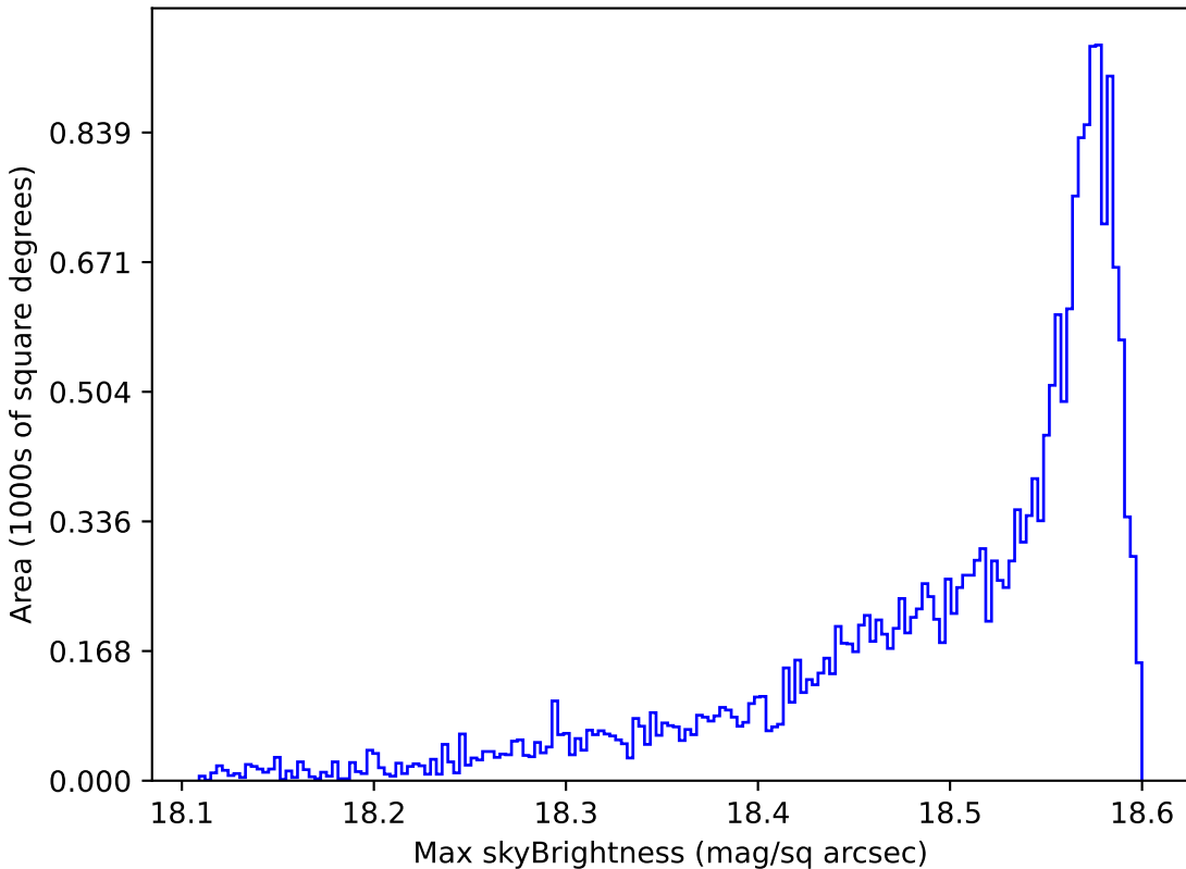
baseline_v3.5_10yrs All sky y band: Max skyBrightness
