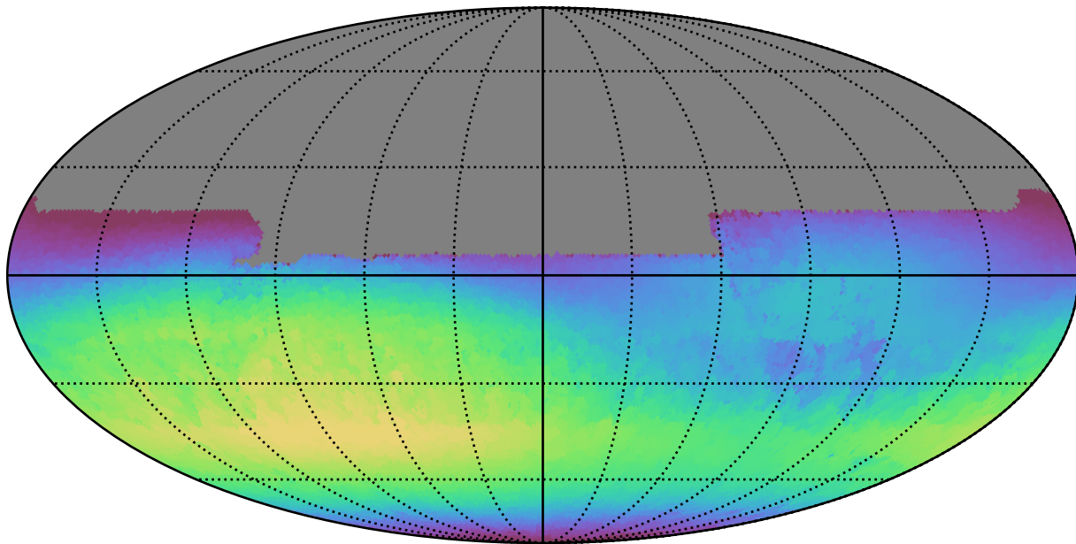
baseline_v3.5_10yrs All sky u band: Max skyBrightness
