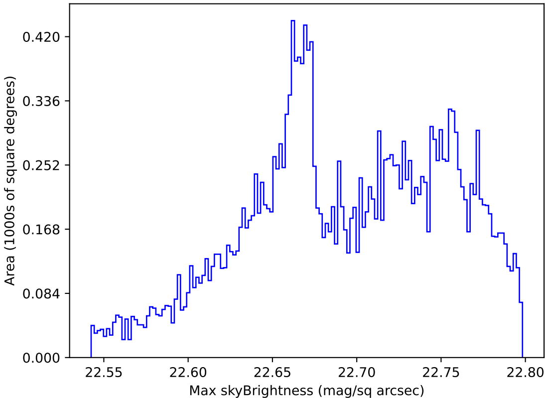
baseline_v3.5_10yrs All sky u band: Max skyBrightness
