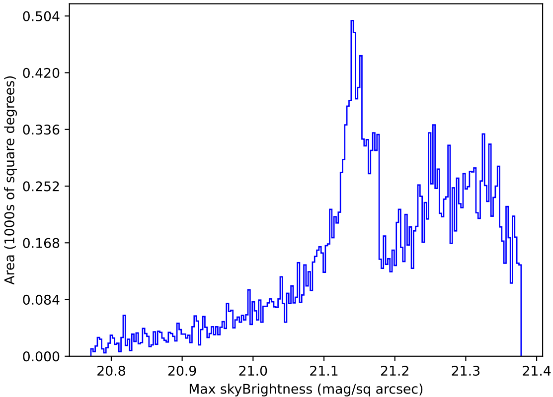
baseline_v3.5_10yrs All sky r band: Max skyBrightness
