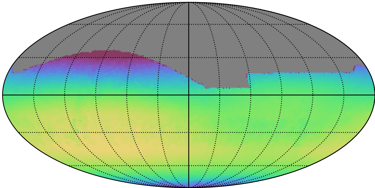
baseline_v3.5_10yrs All sky i band: Max skyBrightness
