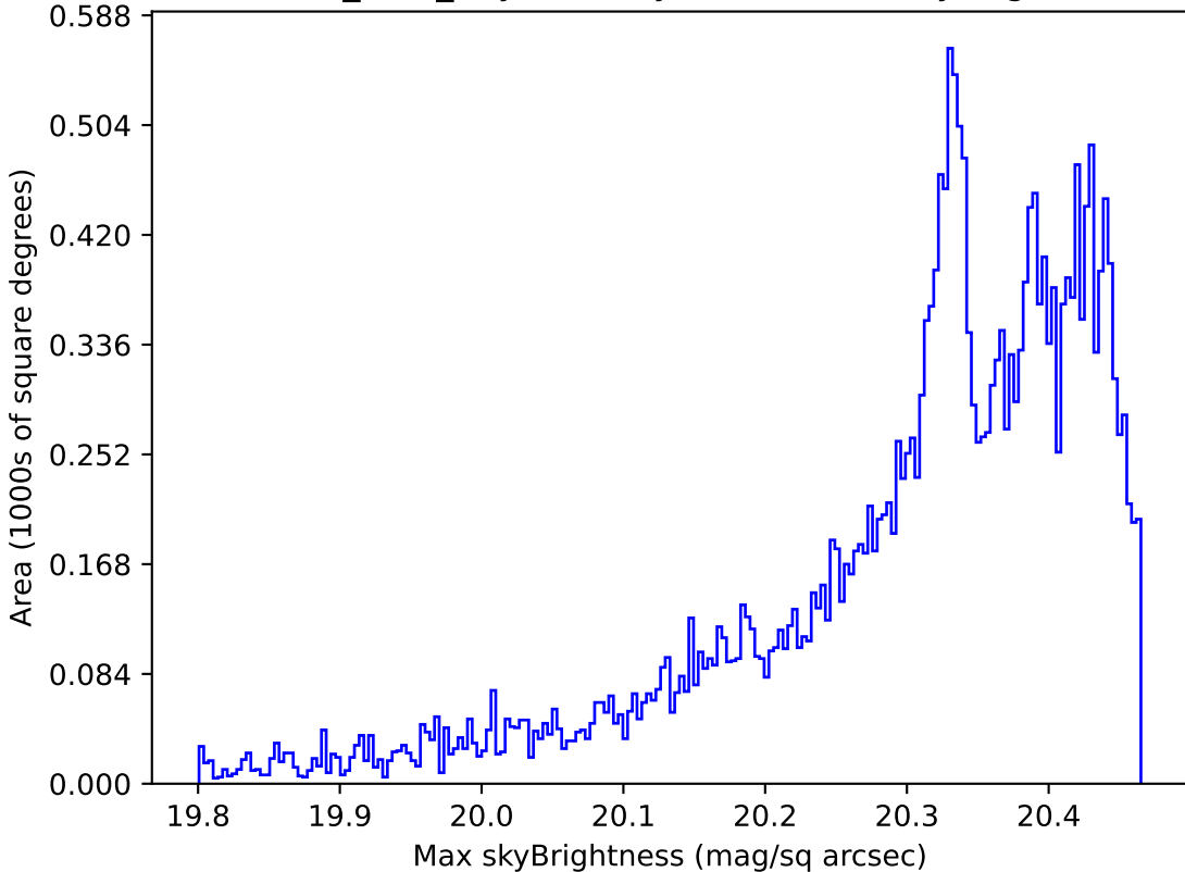
baseline_v3.5_10yrs All sky i band: Max skyBrightness
