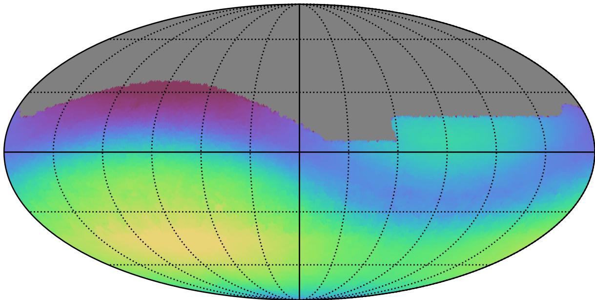
baseline_v3.5_10yrs All sky g band: Max skyBrightness
