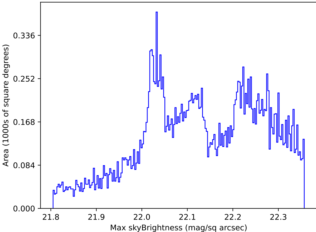
baseline_v3.5_10yrs All sky g band: Max skyBrightness
