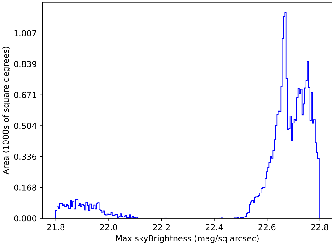
baseline_v3.5_10yrs All sky all bands: Max skyBrightness
