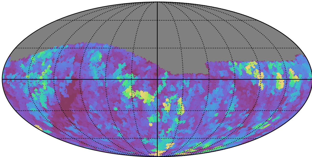
baseline_v3.5_10yrs Yr 1 z band: Max seeingGeom
