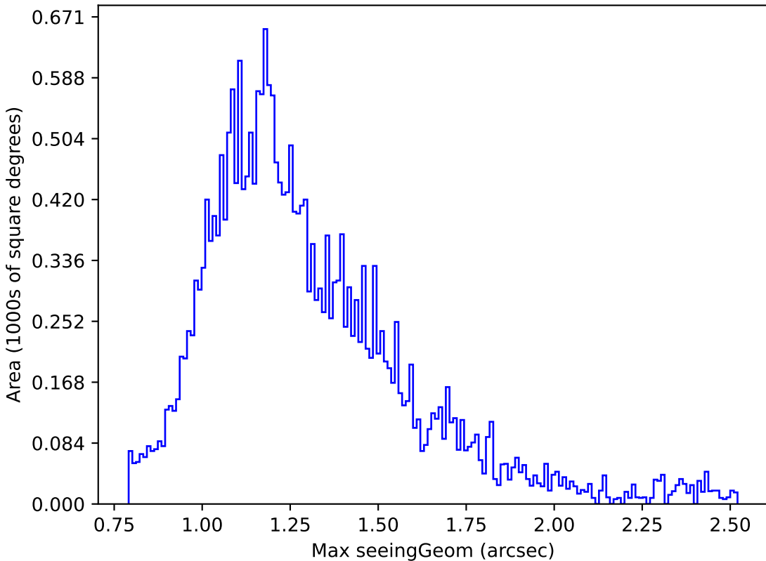
baseline_v3.5_10yrs Yr 1 z band: Max seeingGeom
