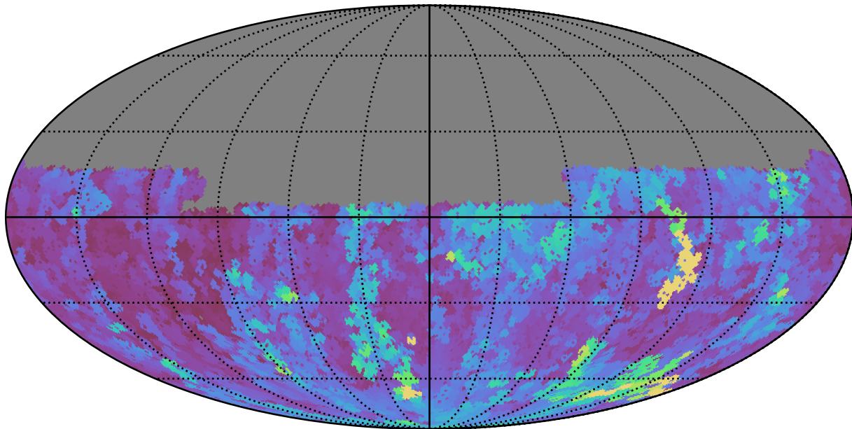
baseline_v3.5_10yrs Yr 1 u band: Max seeingGeom
