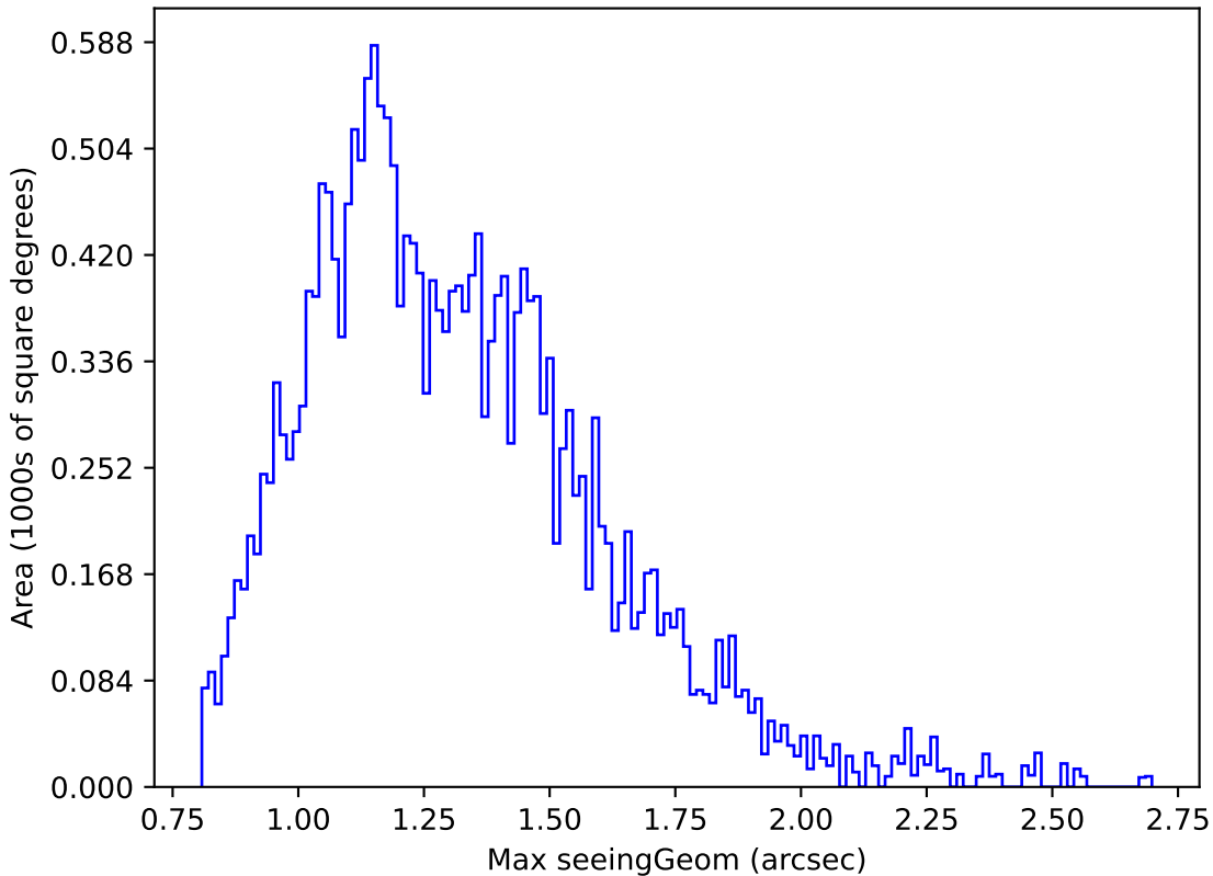
baseline_v3.5_10yrs Yr 1 u band: Max seeingGeom
