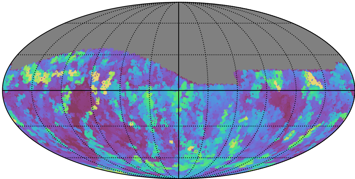
baseline_v3.5_10yrs Yr 1 r band: Max seeingGeom
