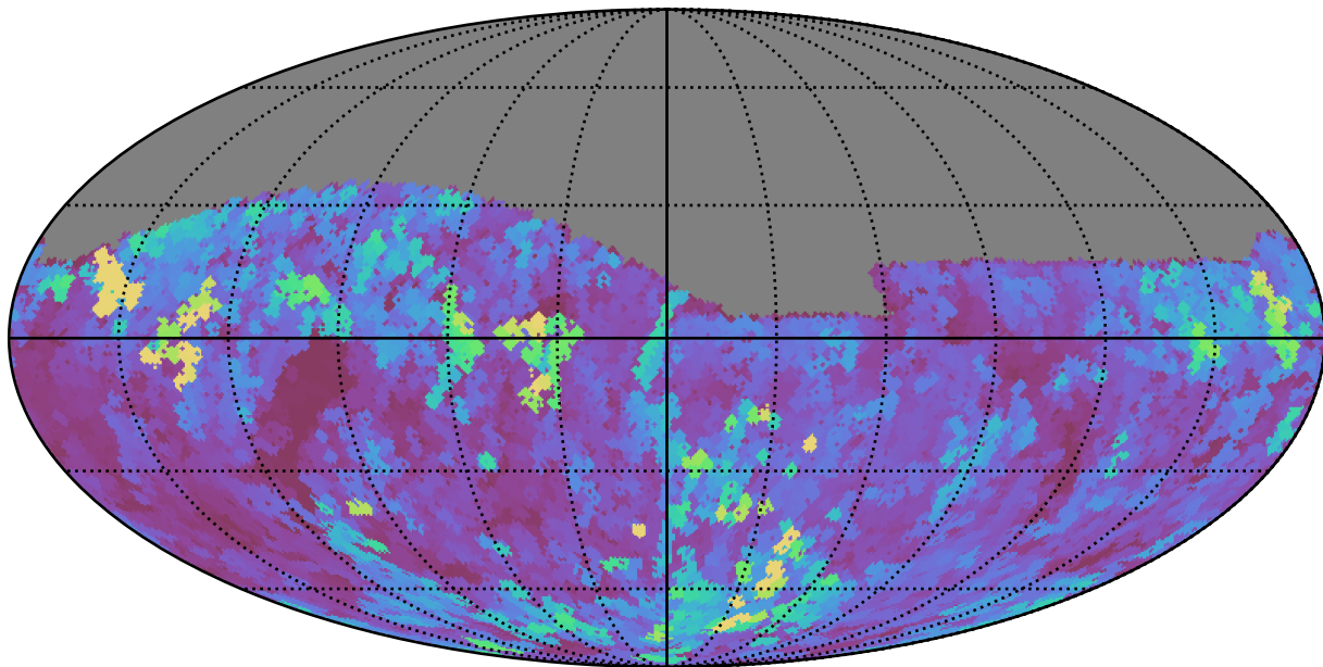
baseline_v3.5_10yrs Yr 1 i band: Max seeingGeom
