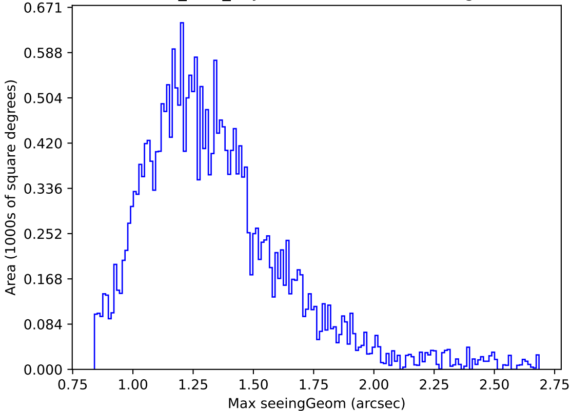
baseline_v3.5_10yrs Yr 1 i band: Max seeingGeom
