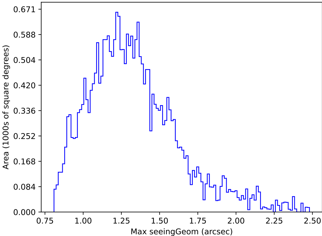
baseline_v3.5_10yrs Yr 1 g band: Max seeingGeom
