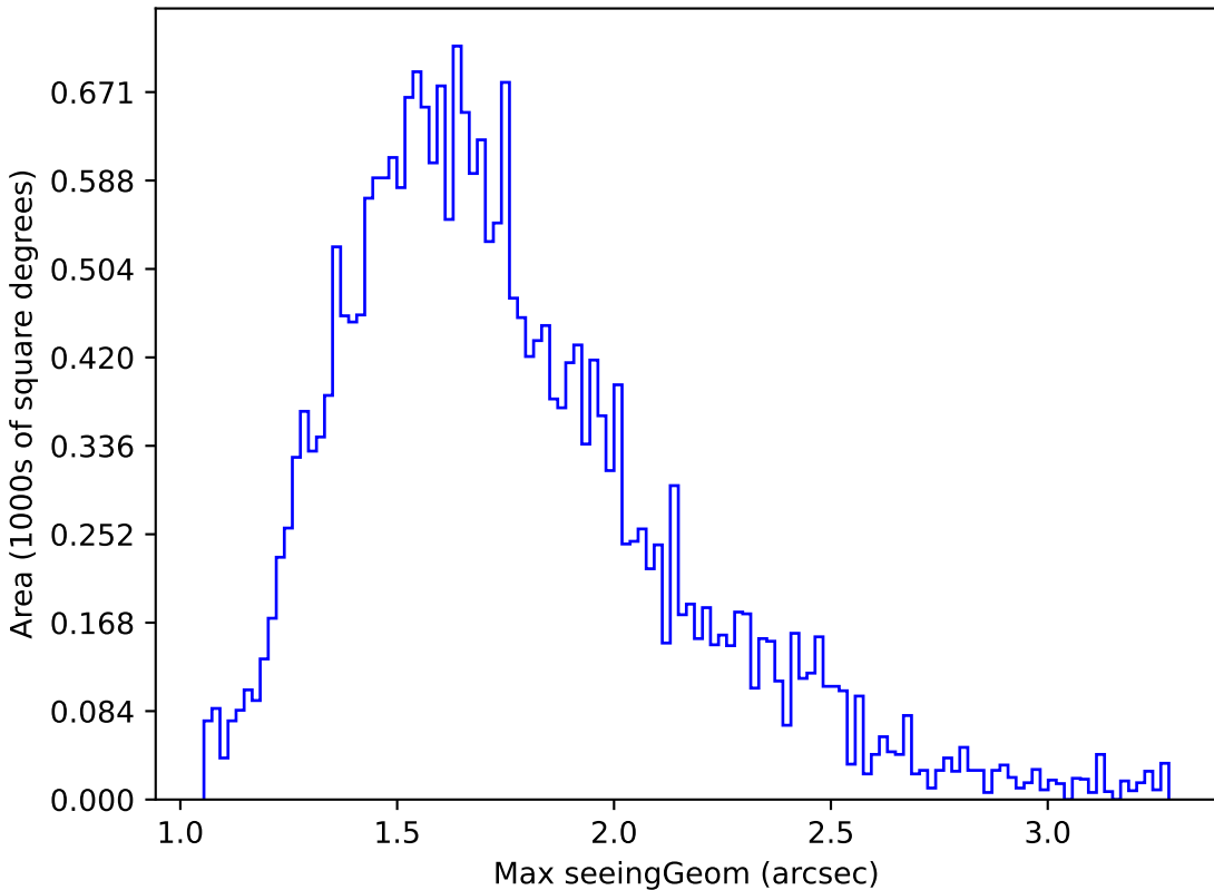
baseline_v3.5_10yrs Yr 1 all bands: Max seeingGeom
