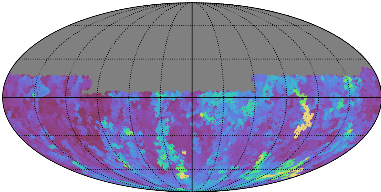
baseline_v3.5_10yrs Yr 1 u band: Max seeingEff
