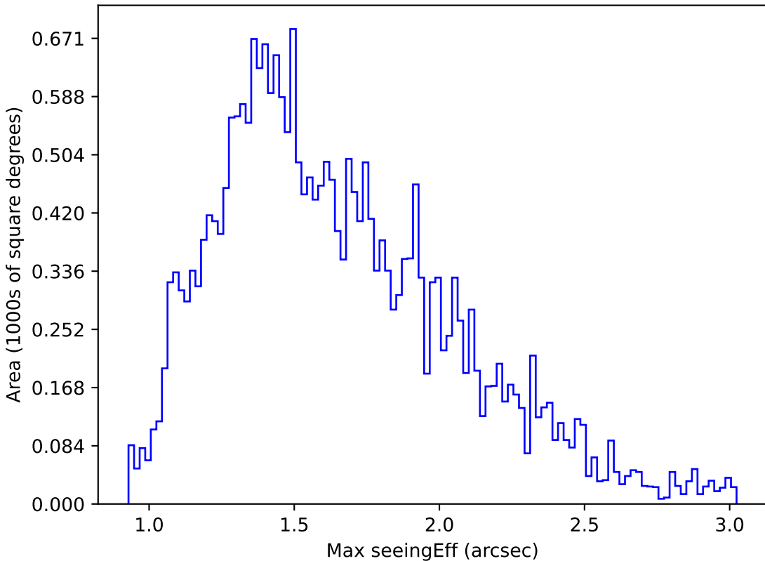
baseline_v3.5_10yrs Yr 1 r band: Max seeingEff
