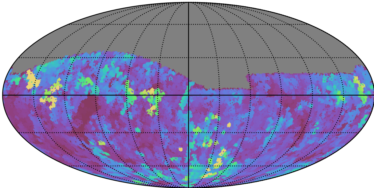
baseline_v3.5_10yrs Yr 1 i band: Max seeingEff
