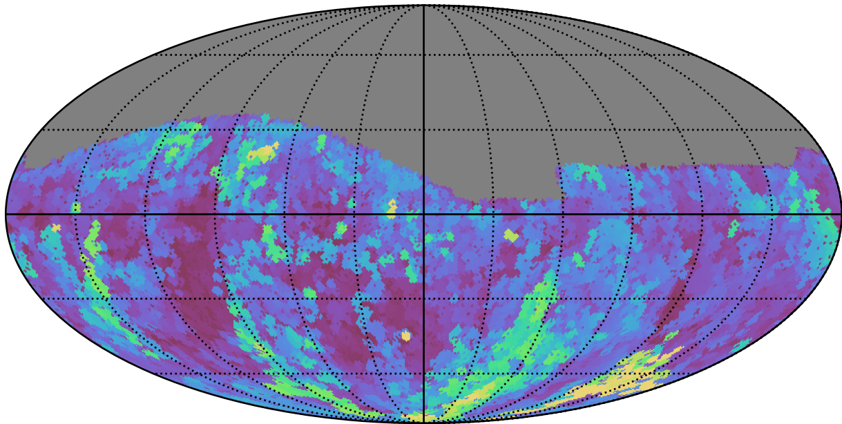
baseline_v3.5_10yrs Yr 1 g band: Max seeingEff
