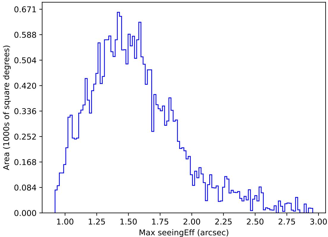
baseline_v3.5_10yrs Yr 1 g band: Max seeingEff
