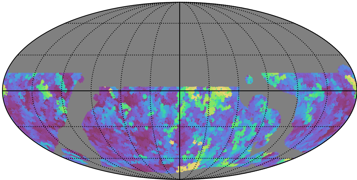
baseline_v3.5_10yrs WFD z band: Max seeingEff
