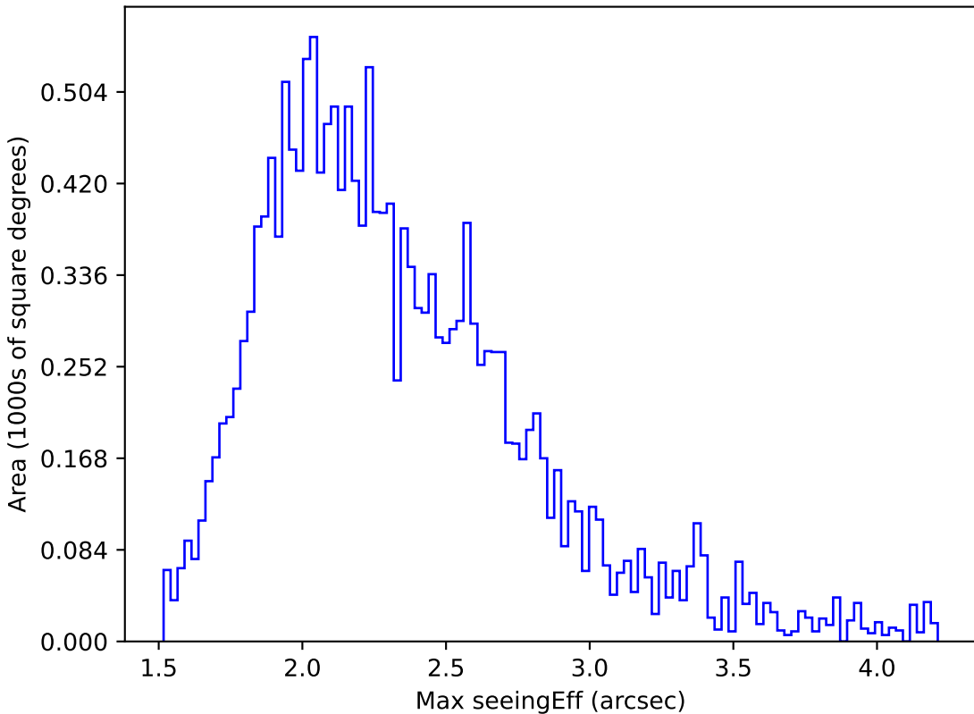
baseline_v3.5_10yrs WFD y band: Max seeingEff
