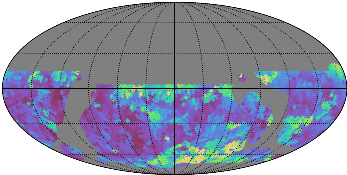
baseline_v3.5_10yrs WFD u band: Max seeingEff
