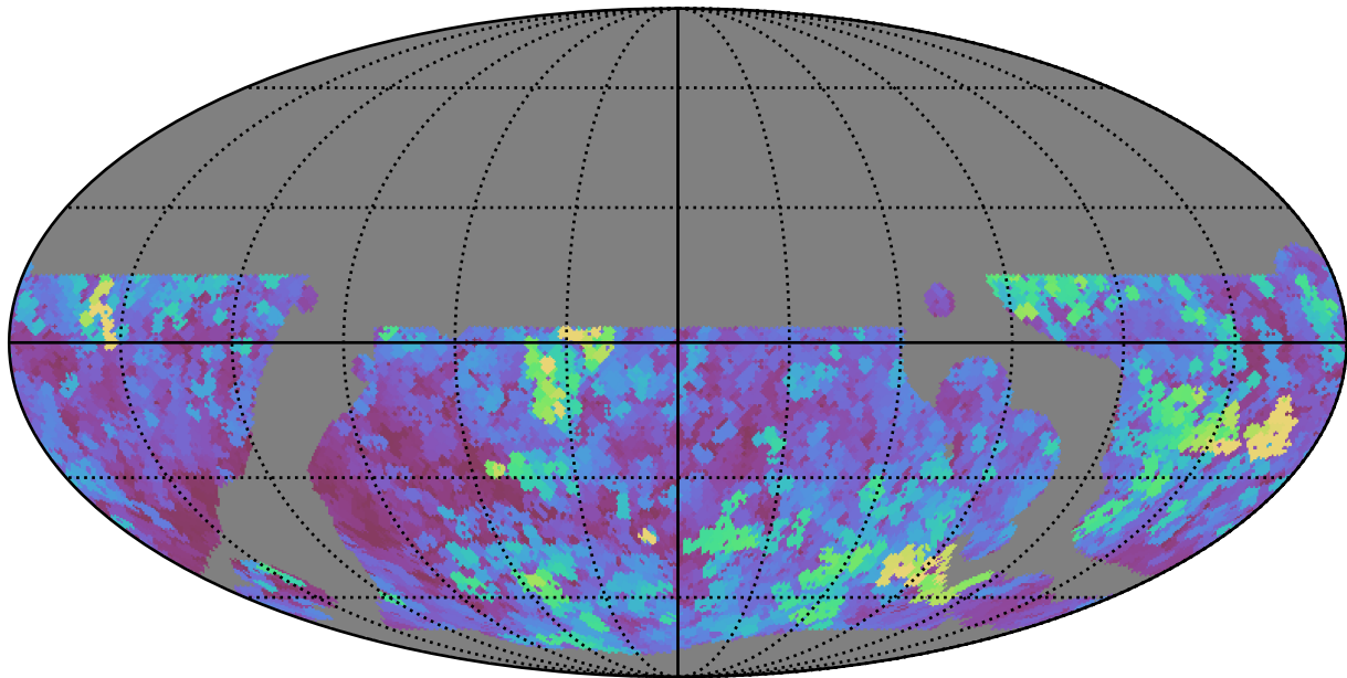
baseline_v3.5_10yrs WFD r band: Max seeingEff
