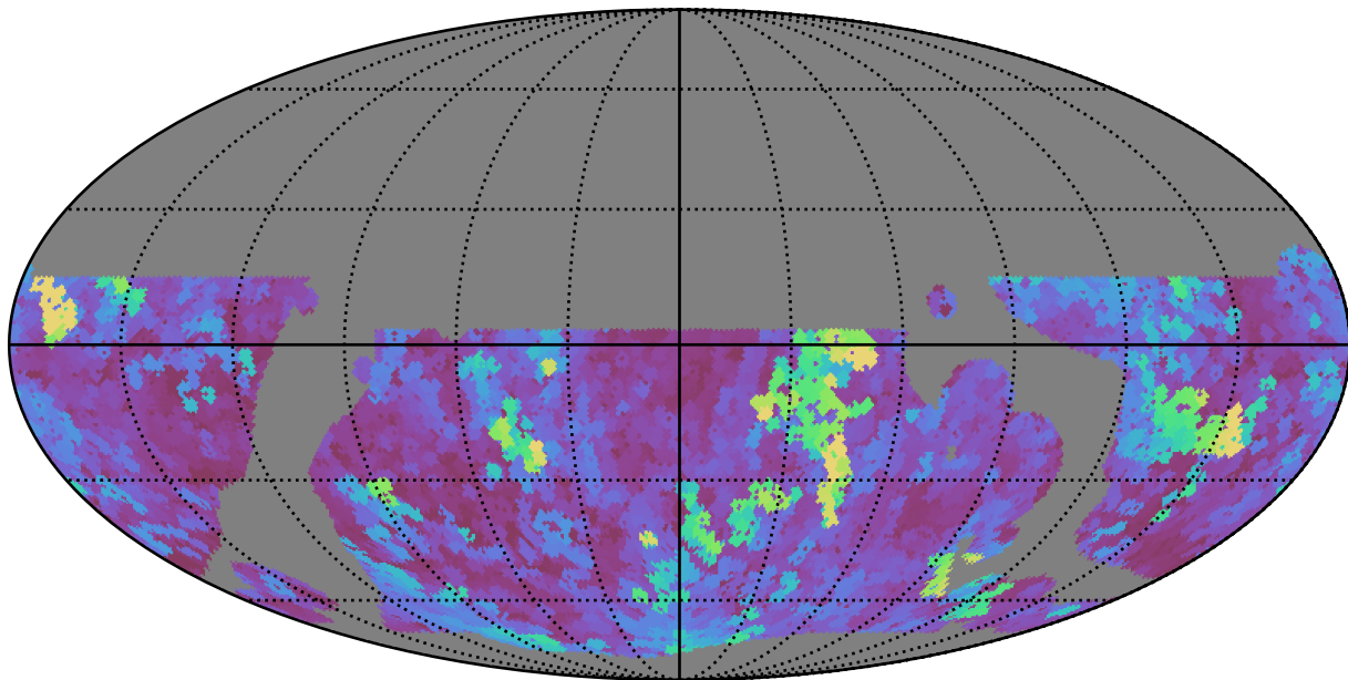
baseline_v3.5_10yrs WFD i band: Max seeingEff
