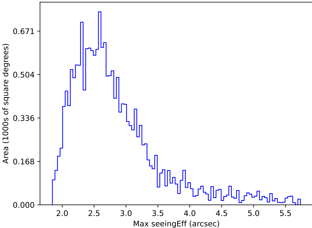
baseline_v3.5_10yrs WFD i band: Max seeingEff
