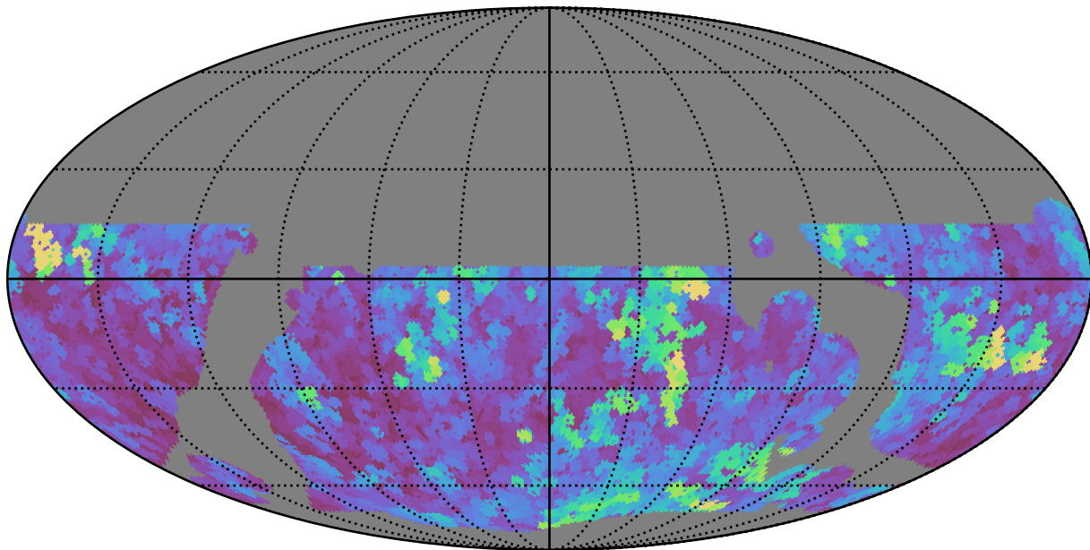
baseline_v3.5_10yrs WFD all bands: Max seeingEff
