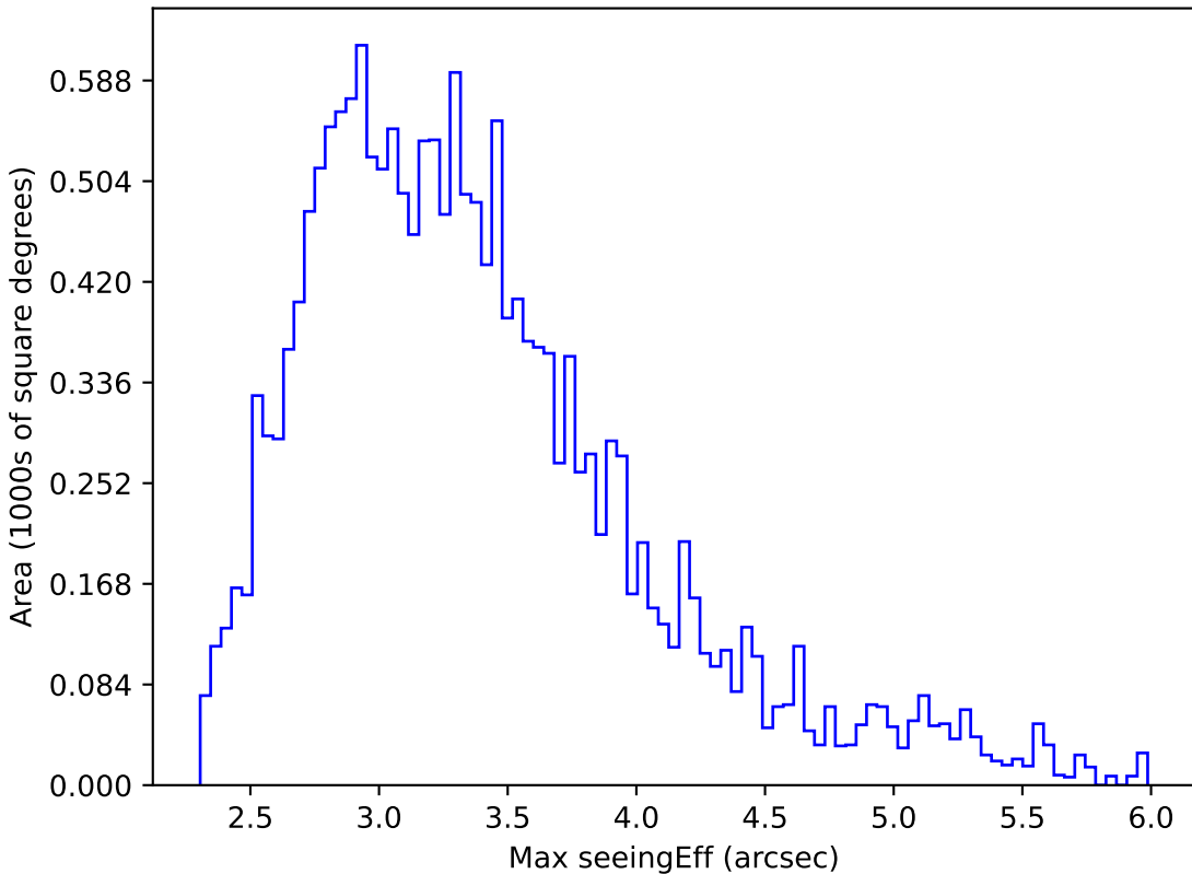
baseline_v3.5_10yrs WFD all bands: Max seeingEff
