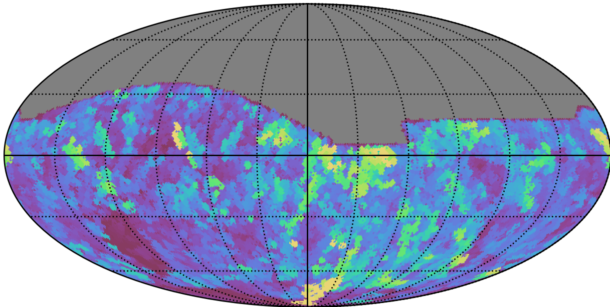
baseline_v3.5_10yrs All sky z band: Max seeingEff
