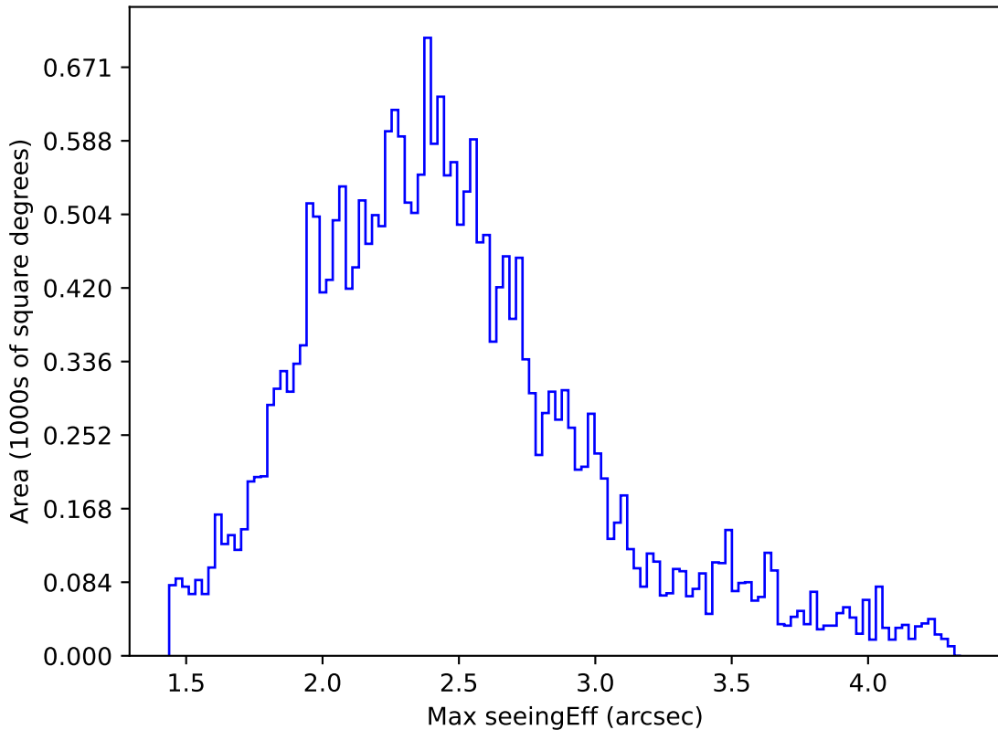
baseline_v3.5_10yrs All sky z band: Max seeingEff
