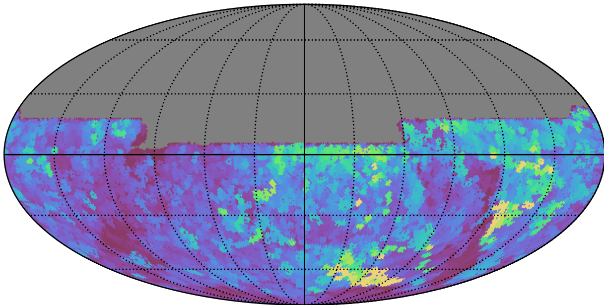
baseline_v3.5_10yrs All sky y band: Max seeingEff
