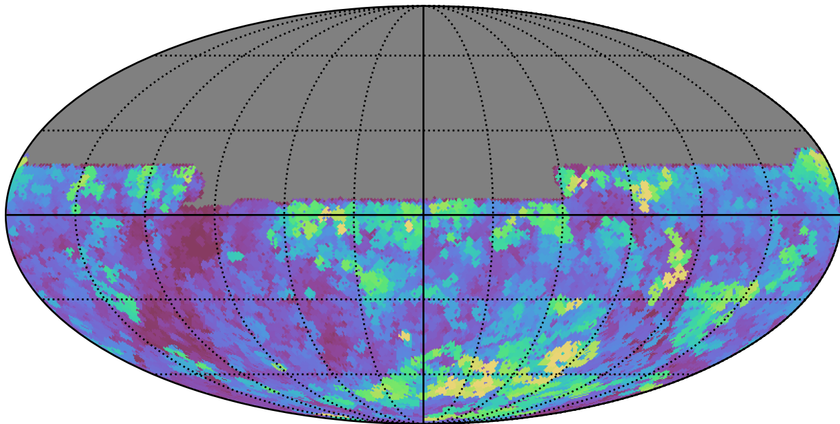
baseline_v3.5_10yrs All sky u band: Max seeingEff
