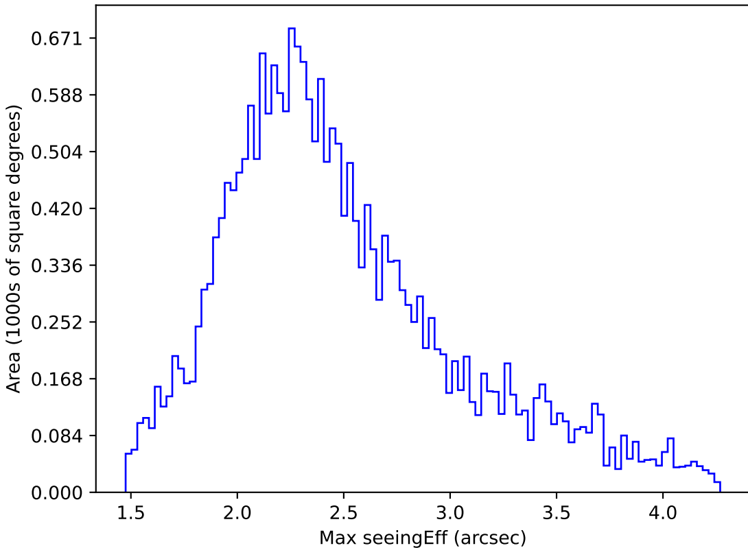
baseline_v3.5_10yrs All sky u band: Max seeingEff
