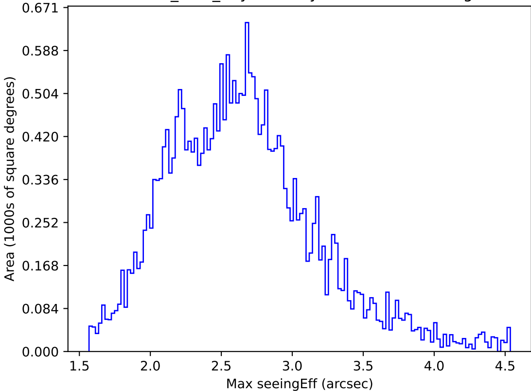
baseline_v3.5_10yrs All sky r band: Max seeingEff
