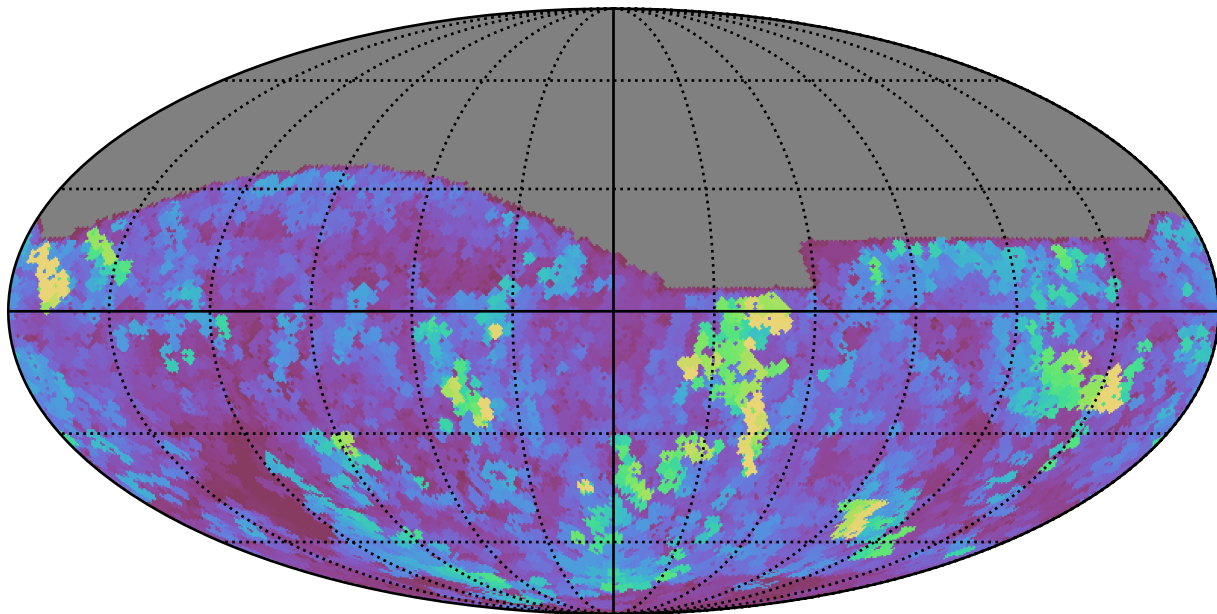
baseline_v3.5_10yrs All sky i band: Max seeingEff
