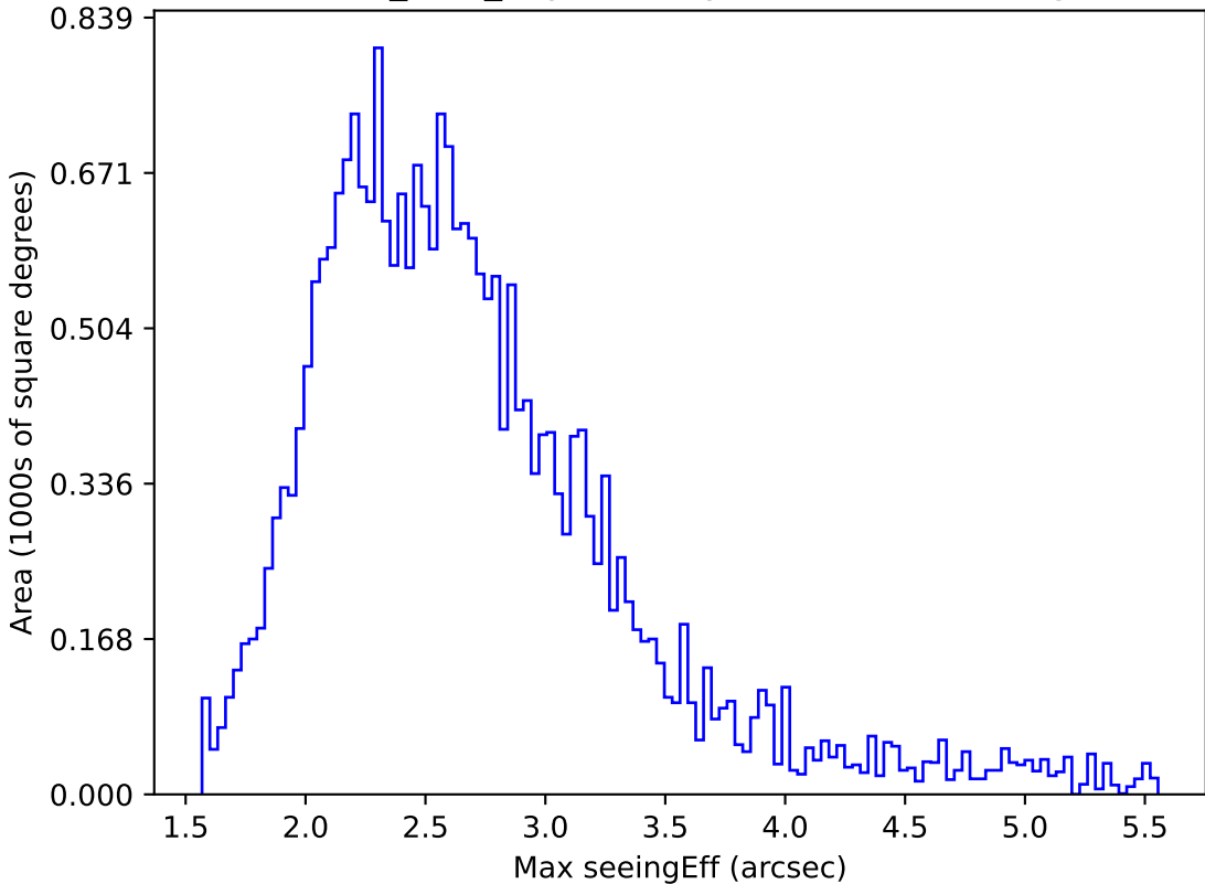
baseline_v3.5_10yrs All sky i band: Max seeingEff
