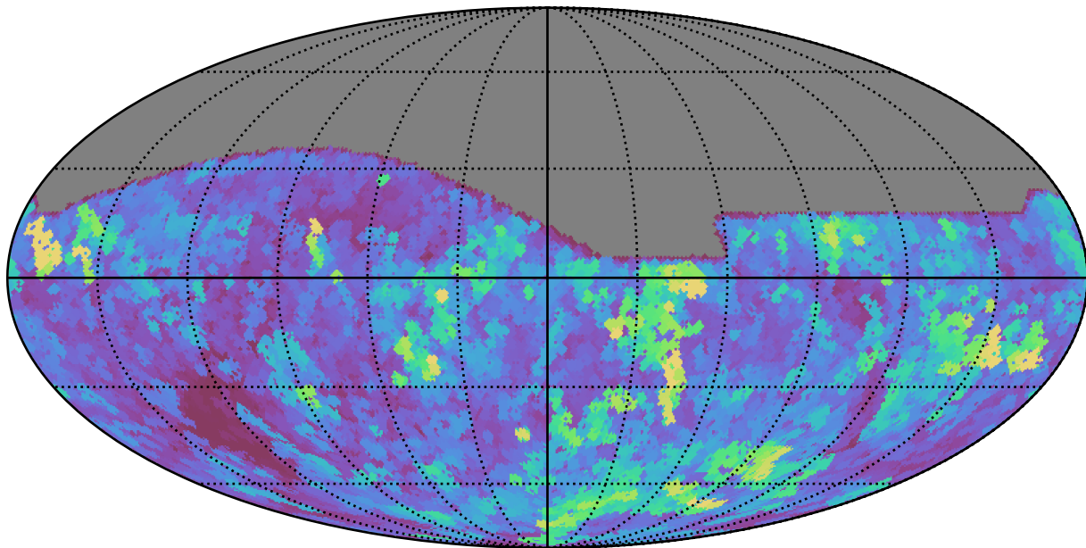
baseline_v3.5_10yrs All sky all bands: Max seeingEff
