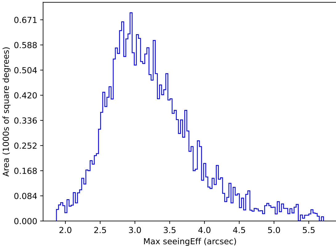
baseline_v3.5_10yrs All sky all bands: Max seeingEff
