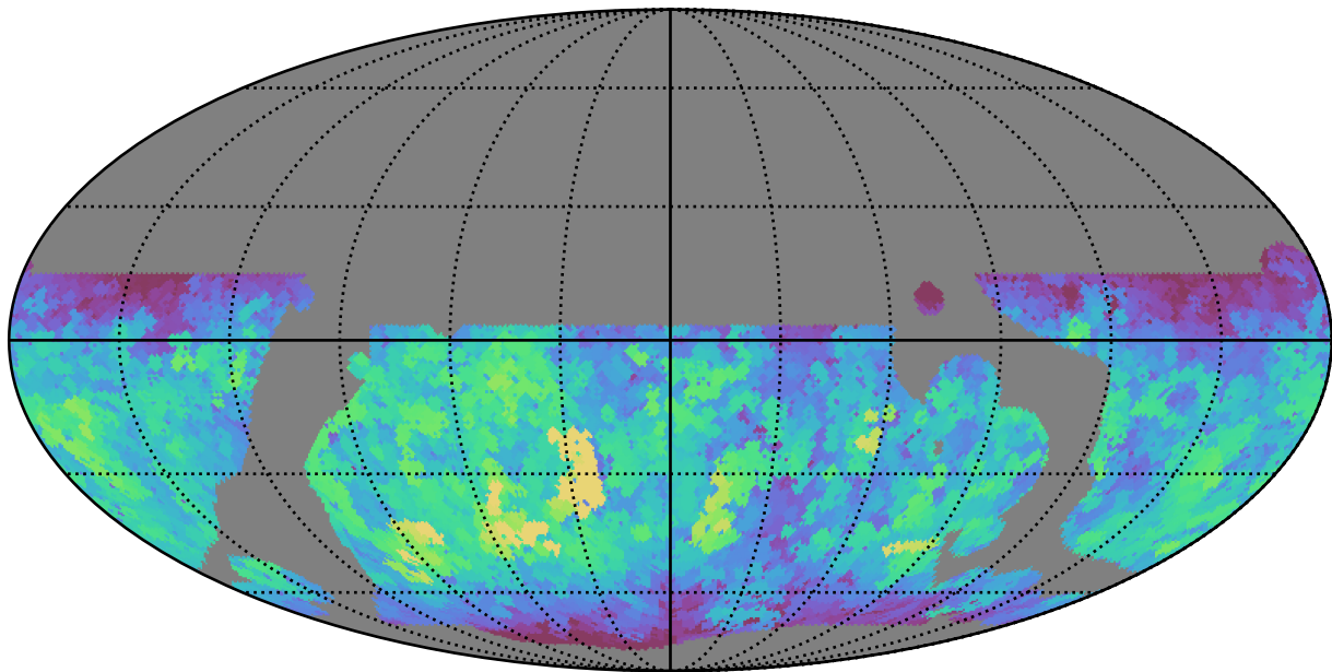
baseline_v3.5_10yrs WFD z band: Max saturation_mag
